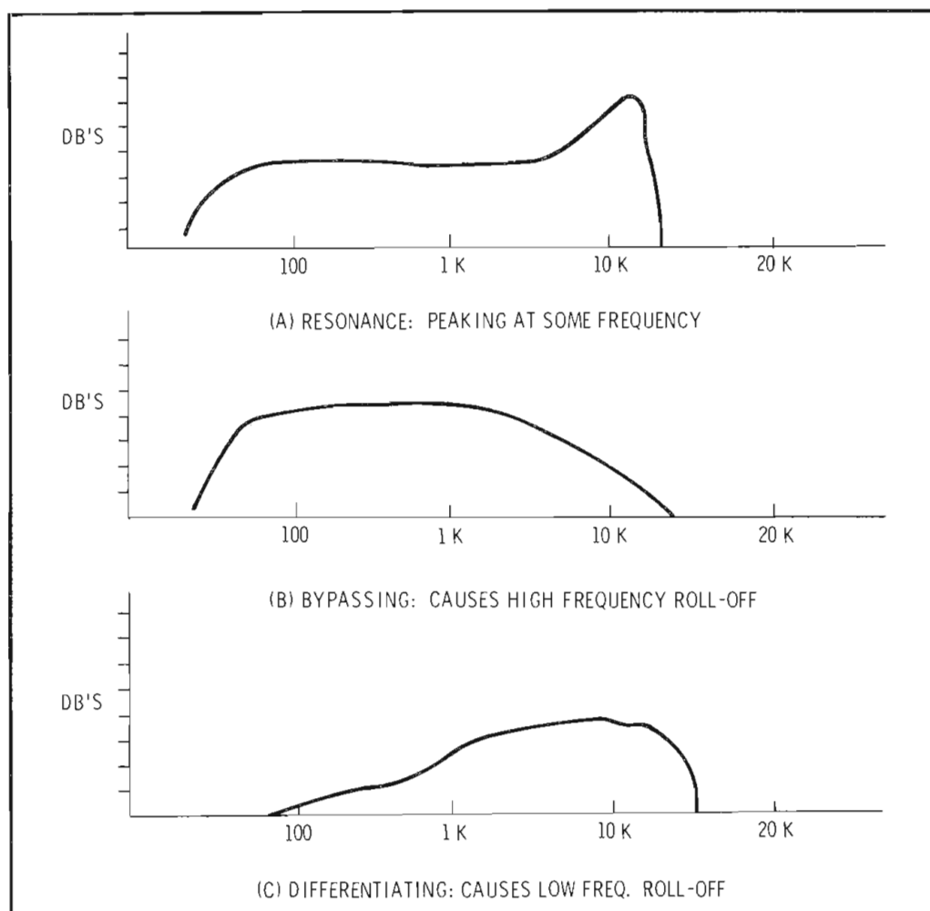
Fig. 1 Various effects the reactive components can have on the signal in a mismatched circuit.
